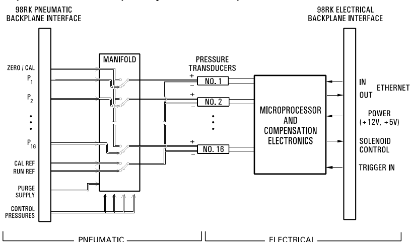
Pneumatic Intelligent Pressure Scanner Functional Diagram
