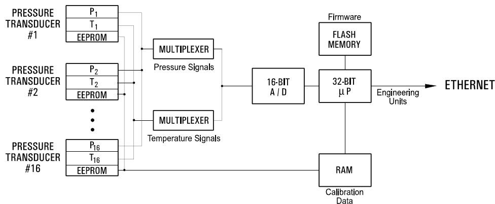
Digital Sensor Temperature Compensation Functional Diagram
